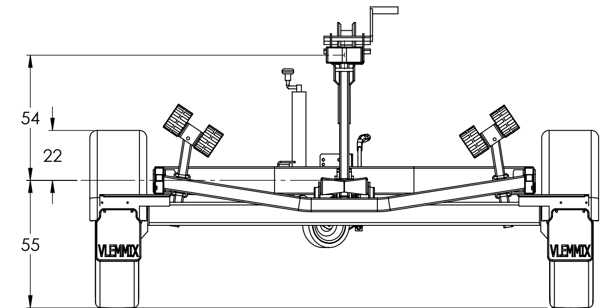
SECTION E-E
